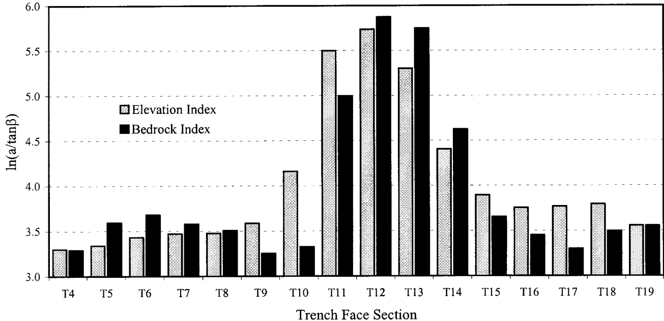
Figure 1. Maimai trench face, distribution of topographic indices for both the elevation (surface topography) and bedrock-derived surfaces
