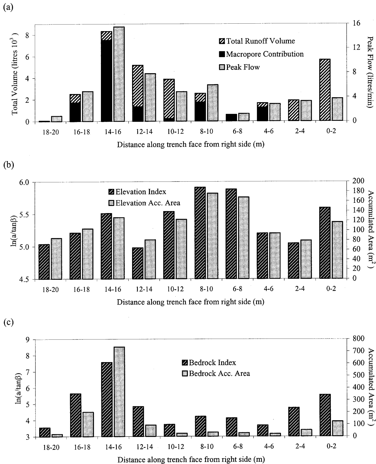
Figure 2. Panola trench face, comparison of digital terrain analysis results with observed cumulative flow for the 6 March event. (a) Observed cumulative volume and peak flow. (b) Elevation (surface topography) and (c) bedrock derived indices
